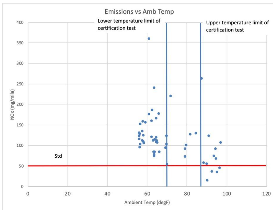
Figure 8: NOx emissions as a function of ambient temperature in city driving conditions for 2012 X5 Diesel B. Certification limit shown in red.
