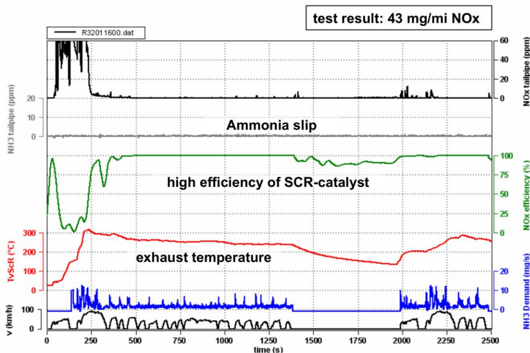
Figure 16: Results from TFP-75 Testing of BMW X5
