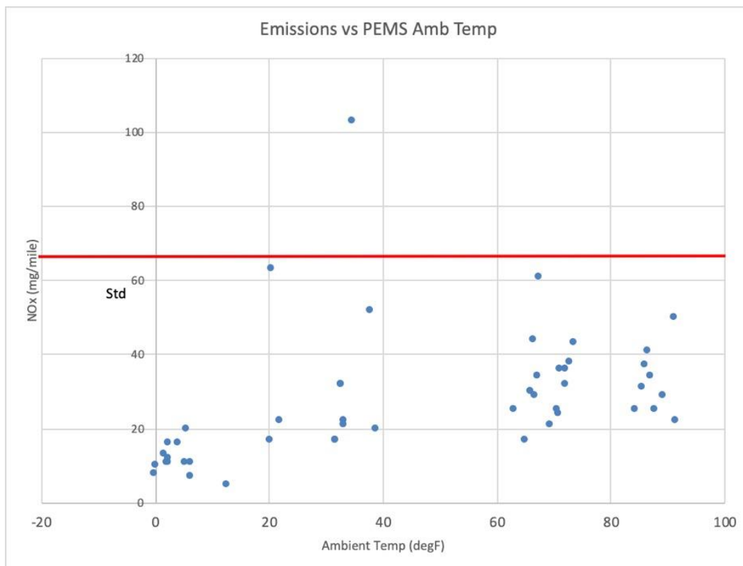
Figure 4: NOx emissions as a function of ambient temperature in city driving conditions for 2012 X5 Gasoline. Certification limit shown in red.
