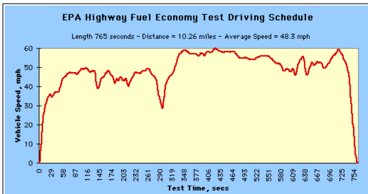
Figure 2: HWFET emissions test cycle.
