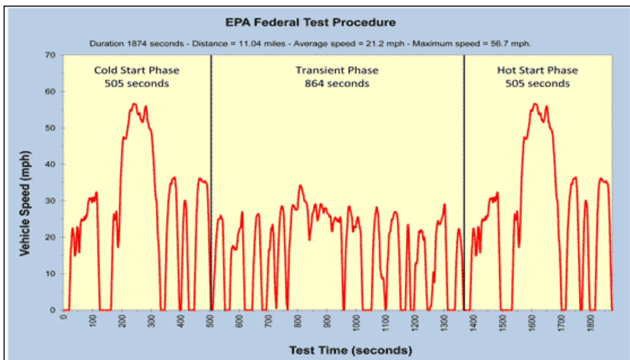
Figure 1: FTP-75 emissions test cycle.
