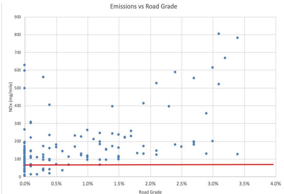
Figure 18: NOx emissions as a function of road grade for 2012 X5 Diesel A. Red line shows the emission standard.
