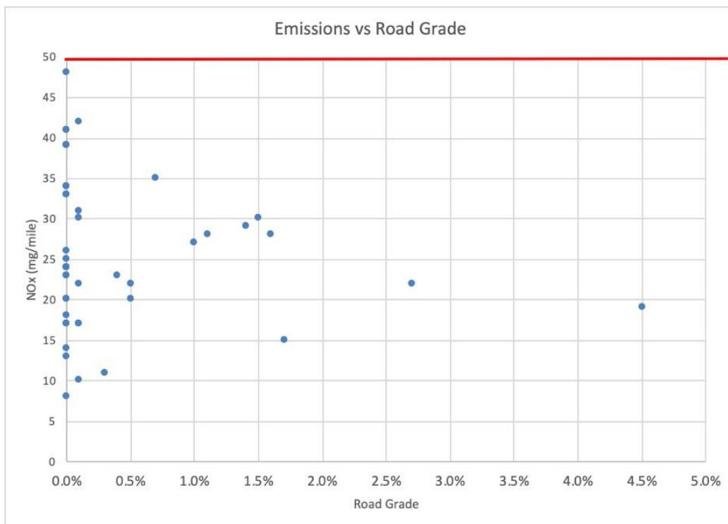
Figure 23: NOx emissions as a function of road grade for 2012 X5 Gasoline. Red line shows the emission standard.
