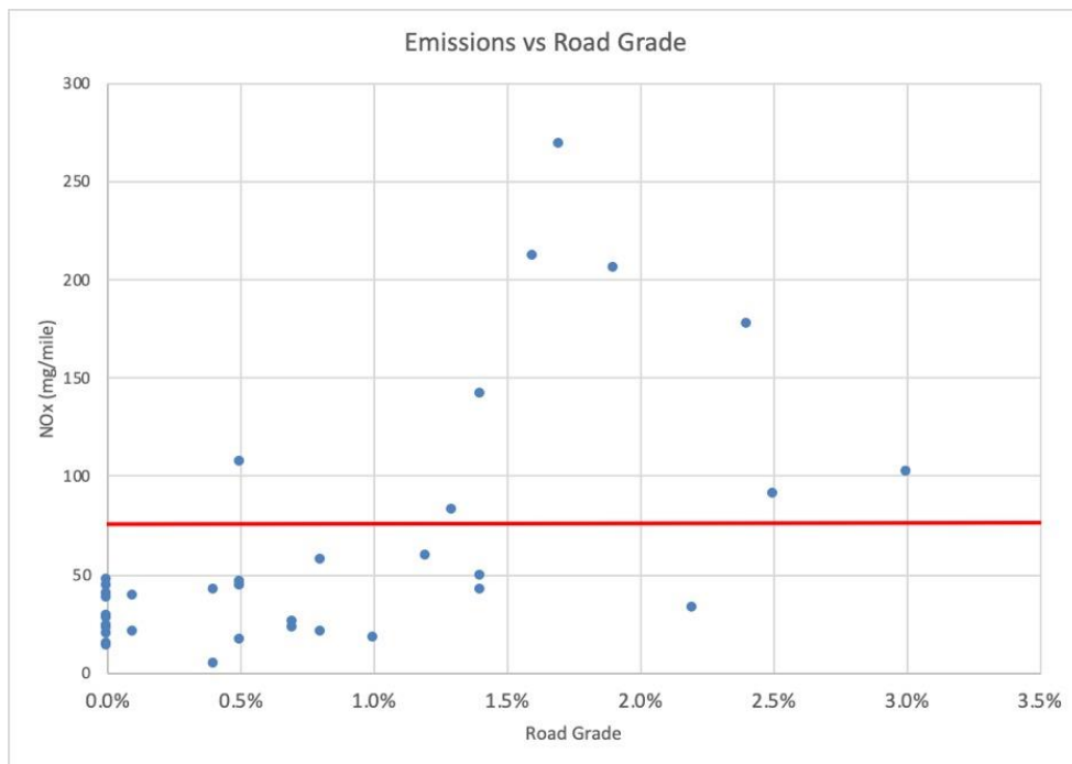
Figure 22: NOx emissions as a function of road grade for 2011 335 Diesel B. Red line shows the emission standard.
